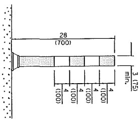
FLEXIBLE DELINEATOR
