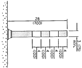
FLEXIBLE DELINEATOR
